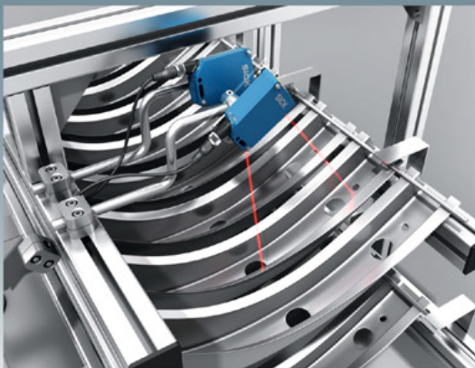
Detection regardless of color or shine. Reliable detection of shiny metal parts, even in an angled detection position.
